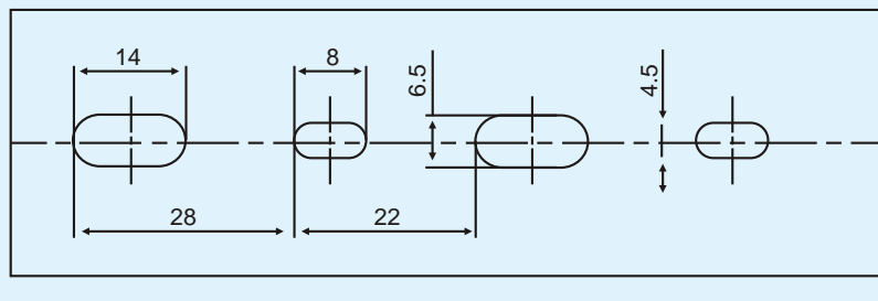
BOTTOM MOUNTING SLOTS FOR ALL SIZES
