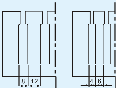
STANDARD SLOT
