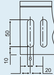
OBLONG SLOT
